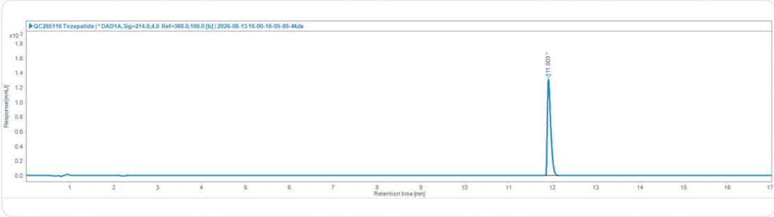
HPLC Chromatogram · Retention Time 11.903 min
